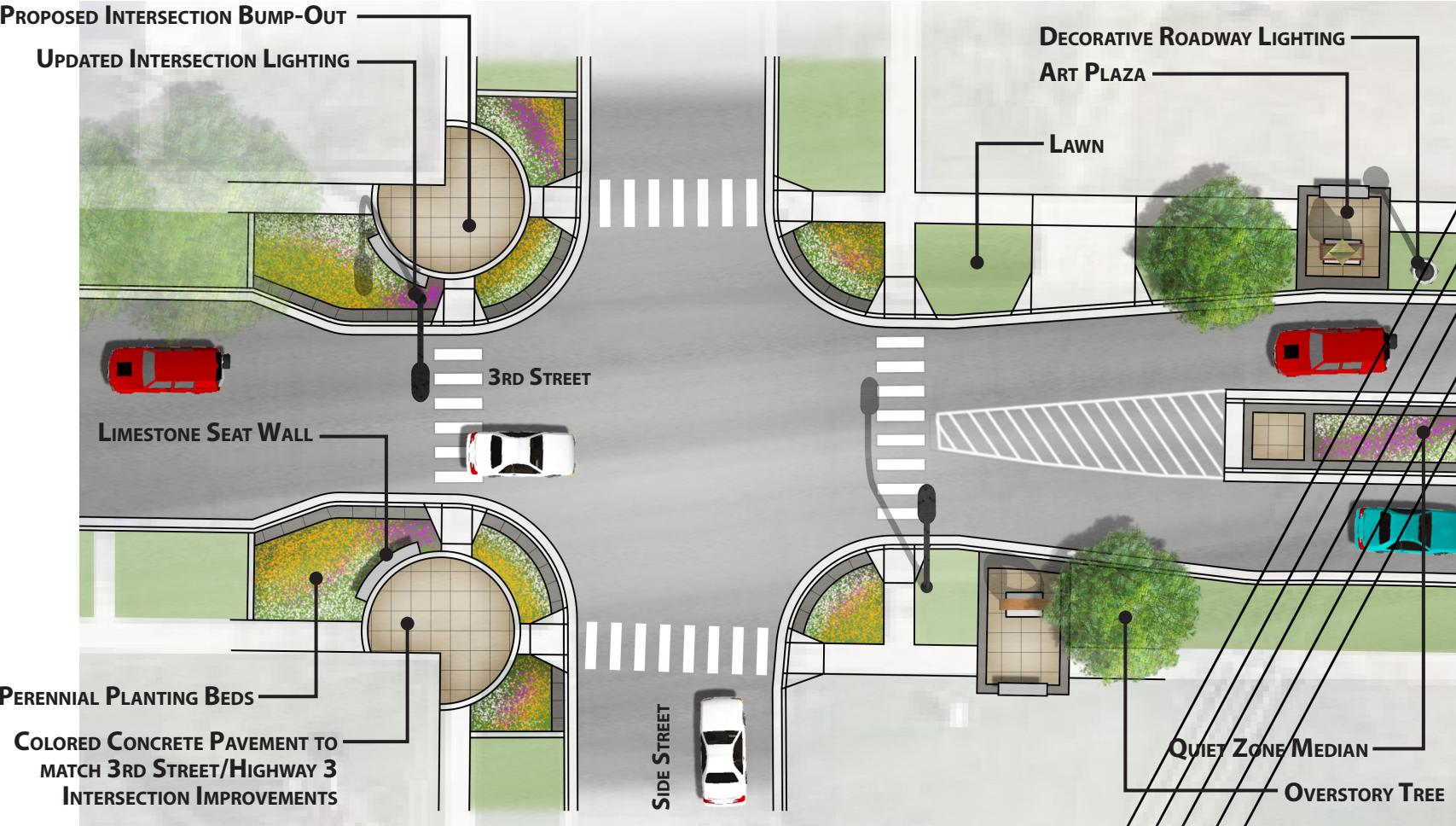
BUMP-OUT TREATMENTS AT POPLAR STREET & LINDEN STREET S.
