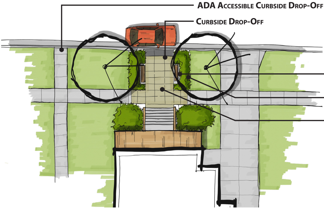
NORTHFIELD ARTS GUILD (NAG) PLAZA CONCEPT PLAN
