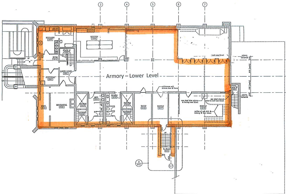
1 LOWER FLOOR PLAN-Remodeling SCALE: Graphical 0 4 8 16 NORTH
