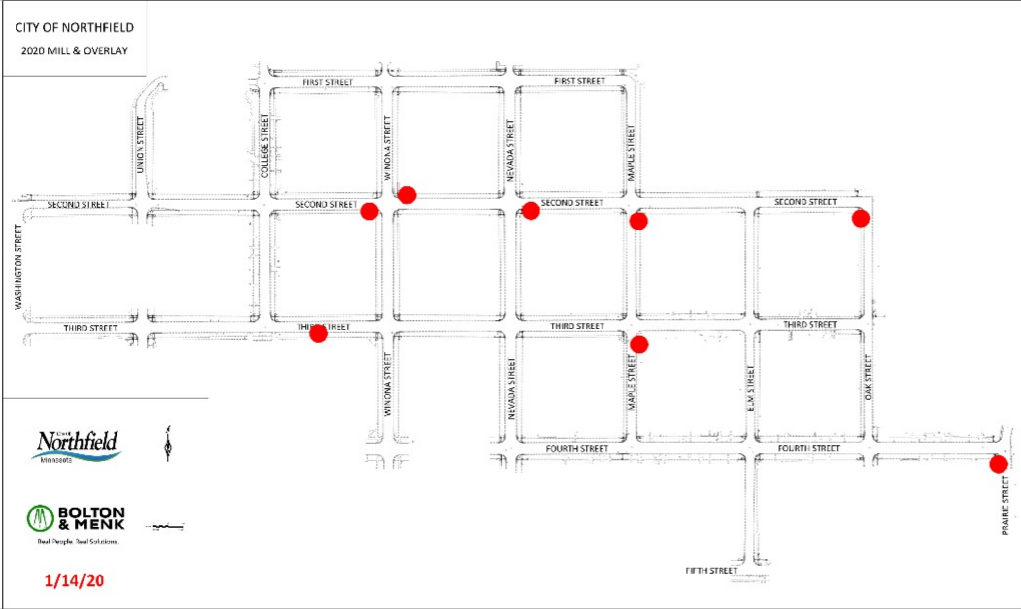
FIGURE 3: PROPOSED ADDITIONAL CATCH BASINS
