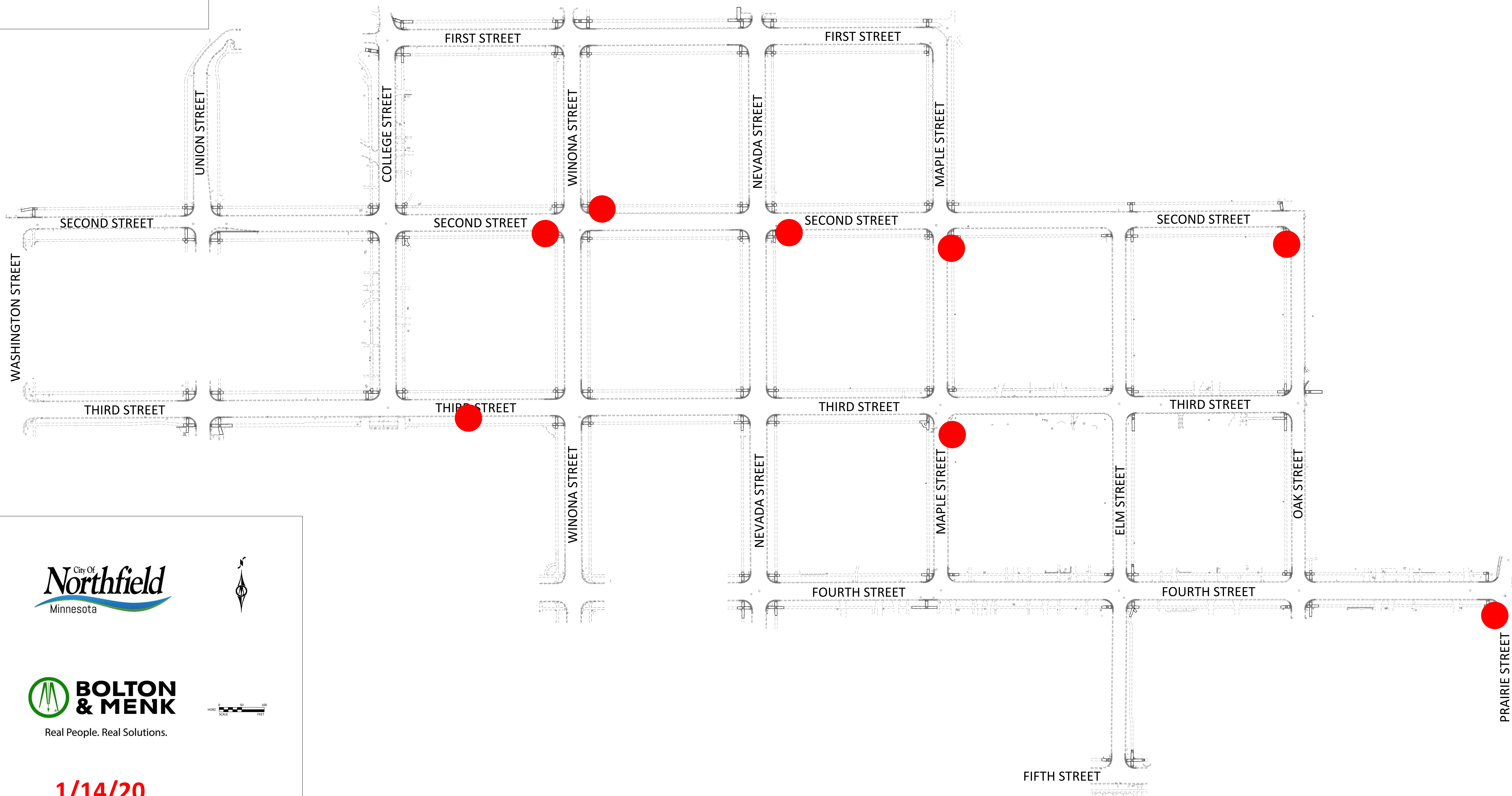
FIGURE 3: PROPOSED ADDITIONAL CATCH BASINS
