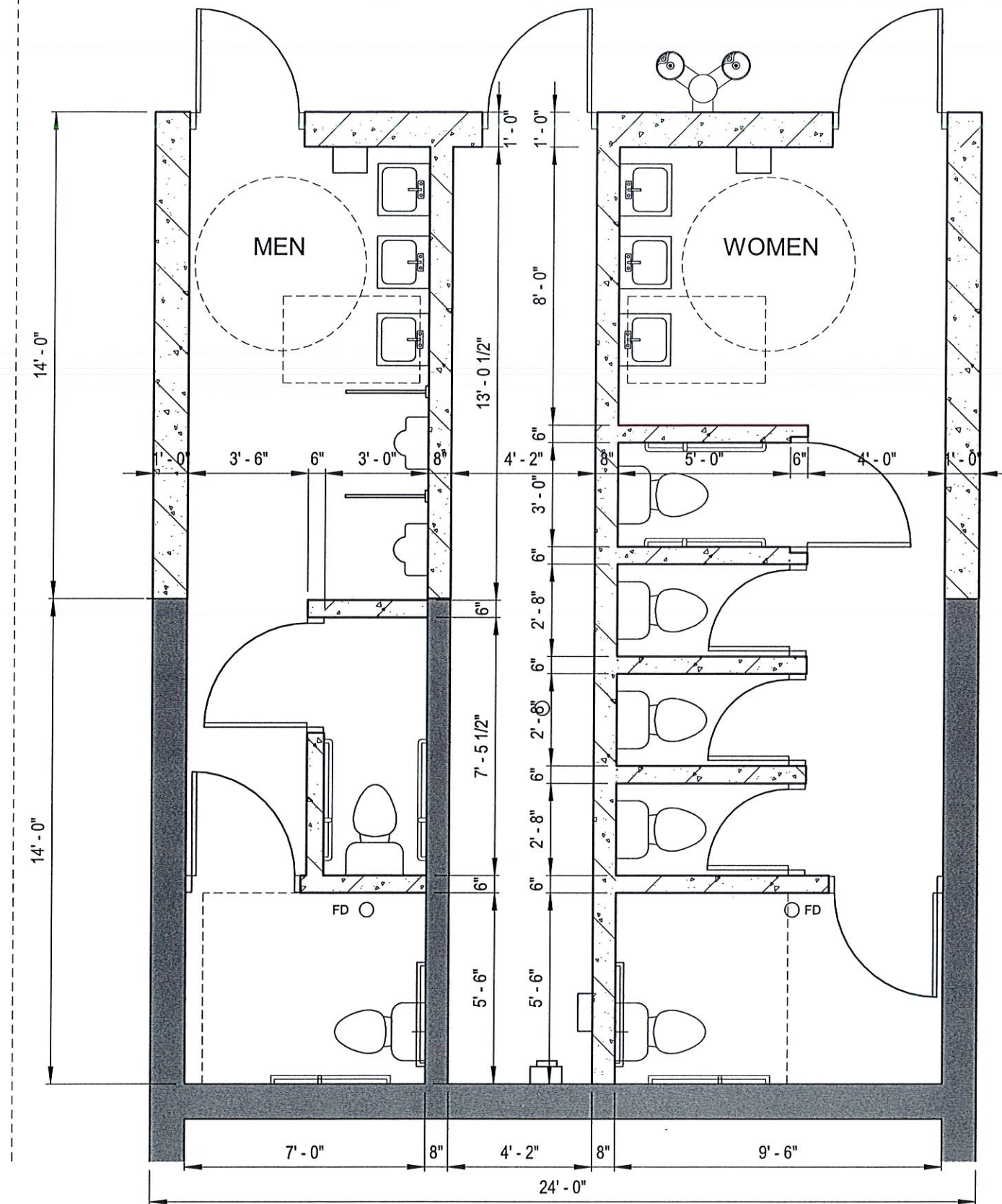
1 SP3 TOILET RM BLDG PLAN 1/4" = 1'-0" OPTION 3
