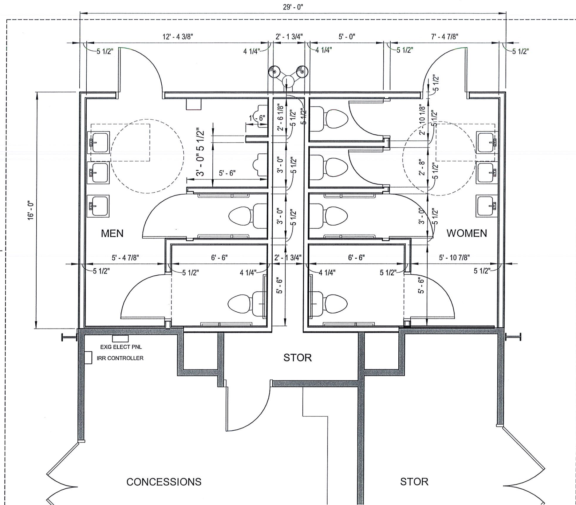
1 PARTIAL CONCESSIONS / TOILET RM BLDG PLAN SC2 1/4" = 1'-0" OPTION 2
