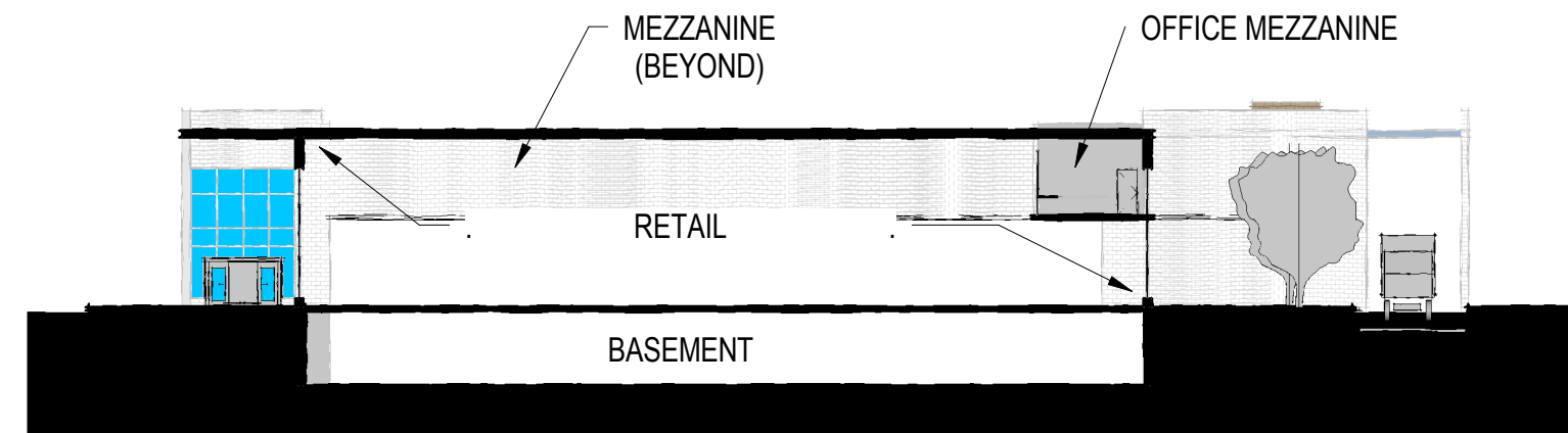
EAST-WEST SECTION showing MEZZANINE and 1/2 BASEMENT
