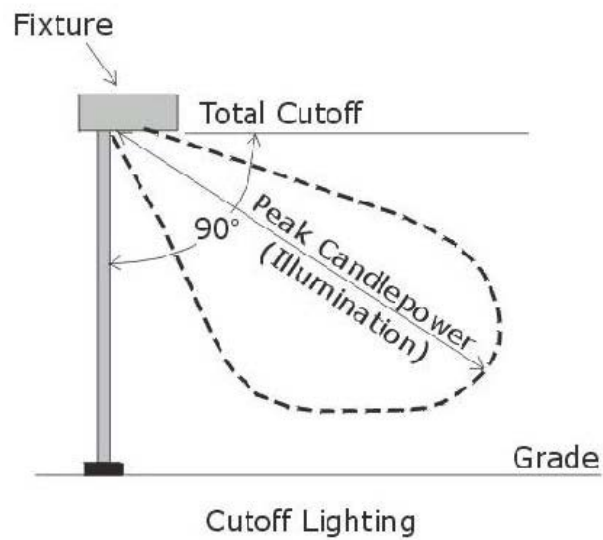
Figure 3-13: Cutoff lighting.
