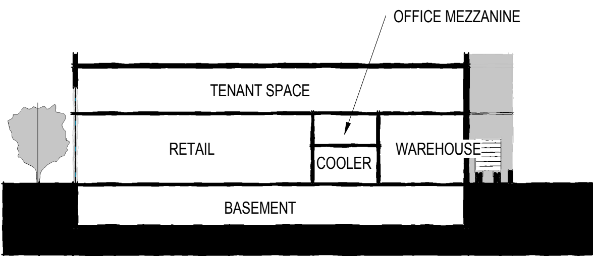
EAST-WEST SECTION showing 2-STORY with FULL BASEMENT
