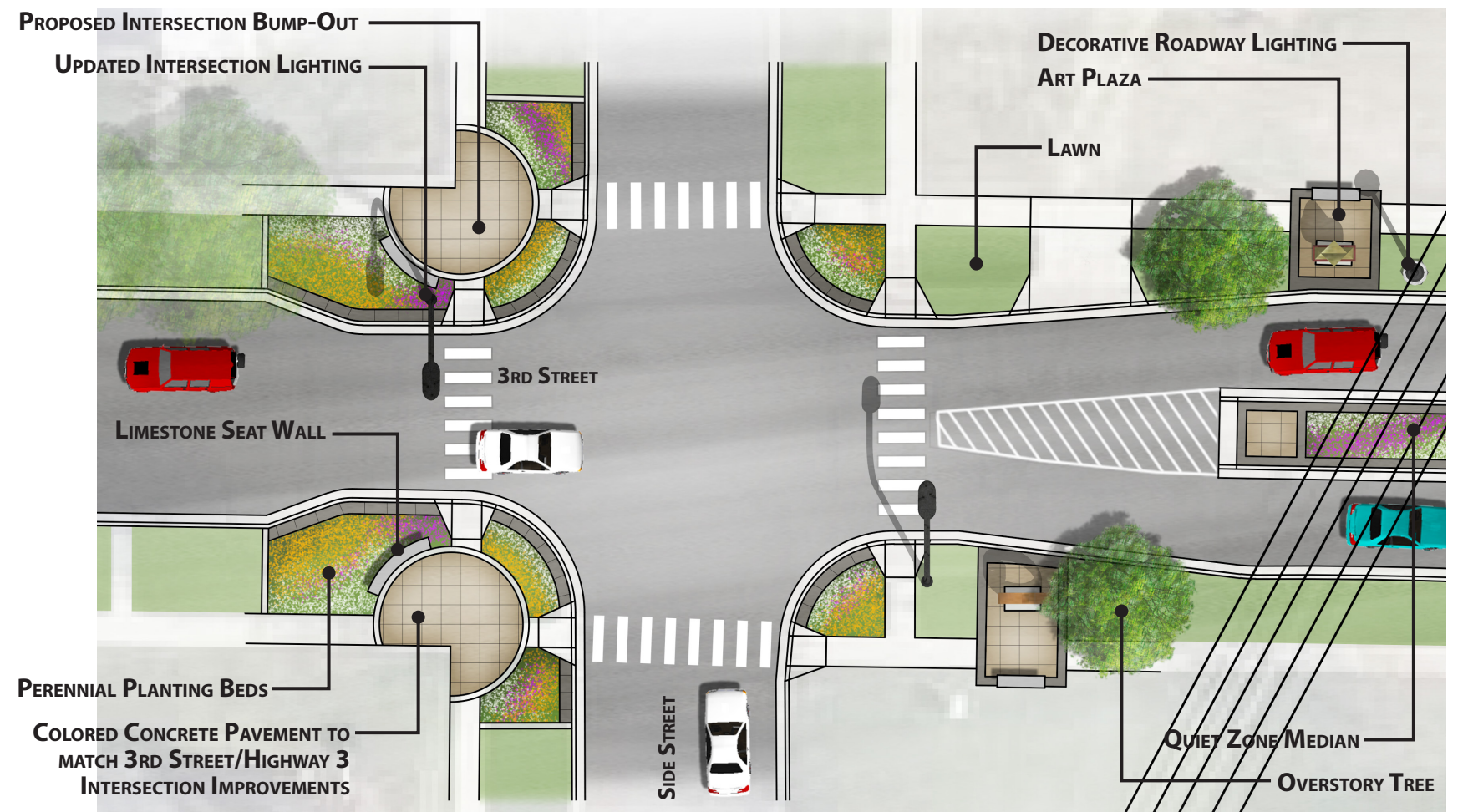
BUMP-OUT TREATMENTS AT POPLAR STREET & LINDEN STREET S.
