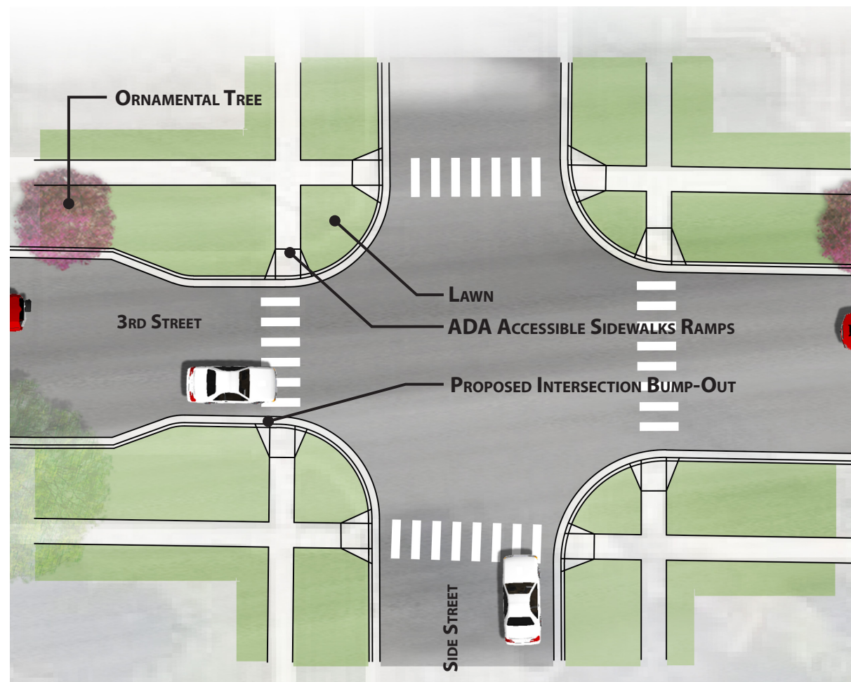
BUMP-OUT TREATMENTS AT ORCHARD STREET S. & PLUM STREET S.
