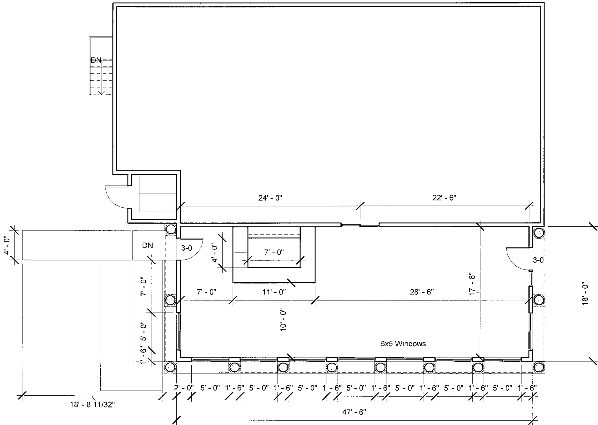
1 Level 1 1/8" = 1'-0"
